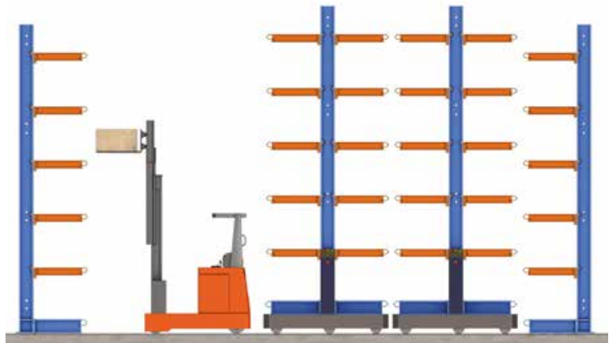
The illustration shows the layout of the cantilever racks on mobile bases and the minimum aisle space needed for forklift manoeuvring.
